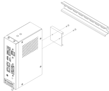
DIN RAIL mounting (included in the package)
