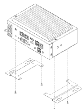
FLAT mounting (optional NOT included)
