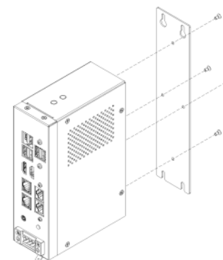
WALL mounting (included in the package)
